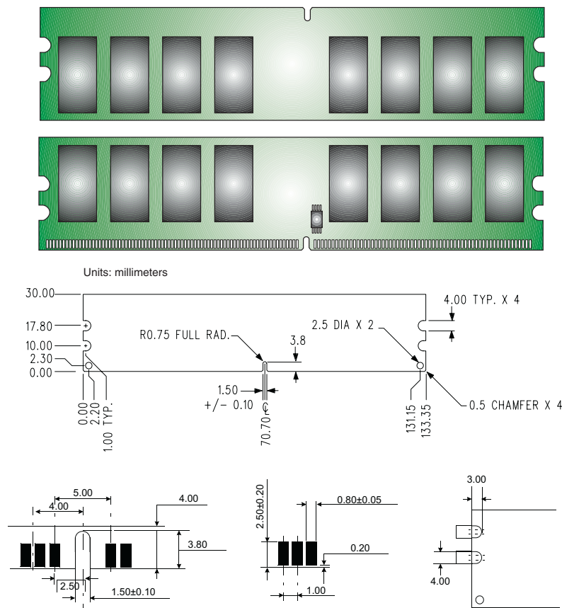
Figure 1: KVR800D2N5/1G 240-Pin DIMM
